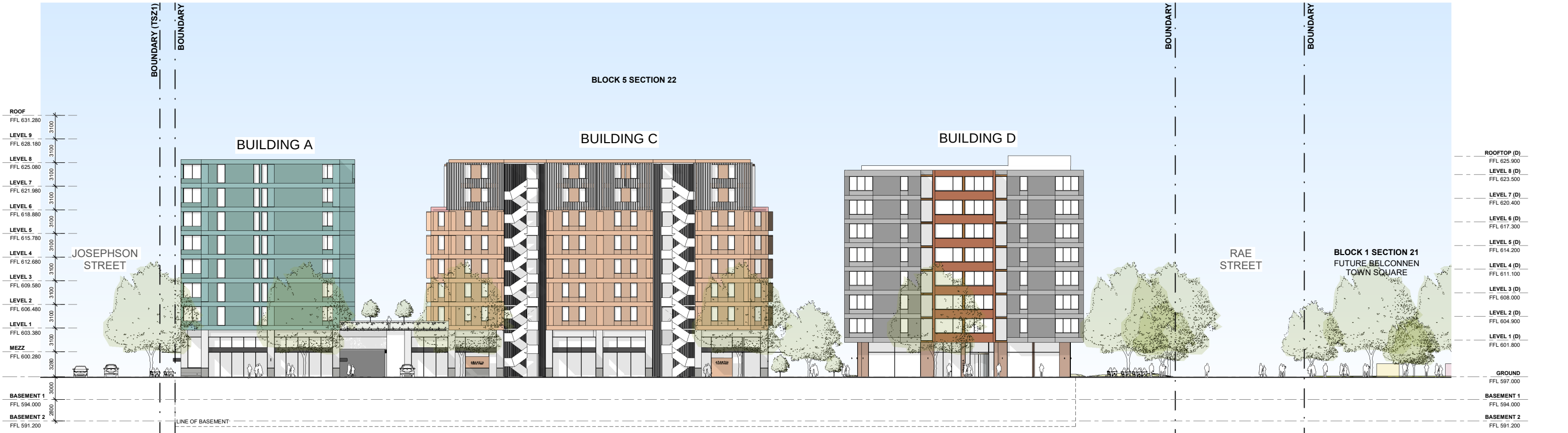
SOUTH ELEVATION - PURDUE STREET
