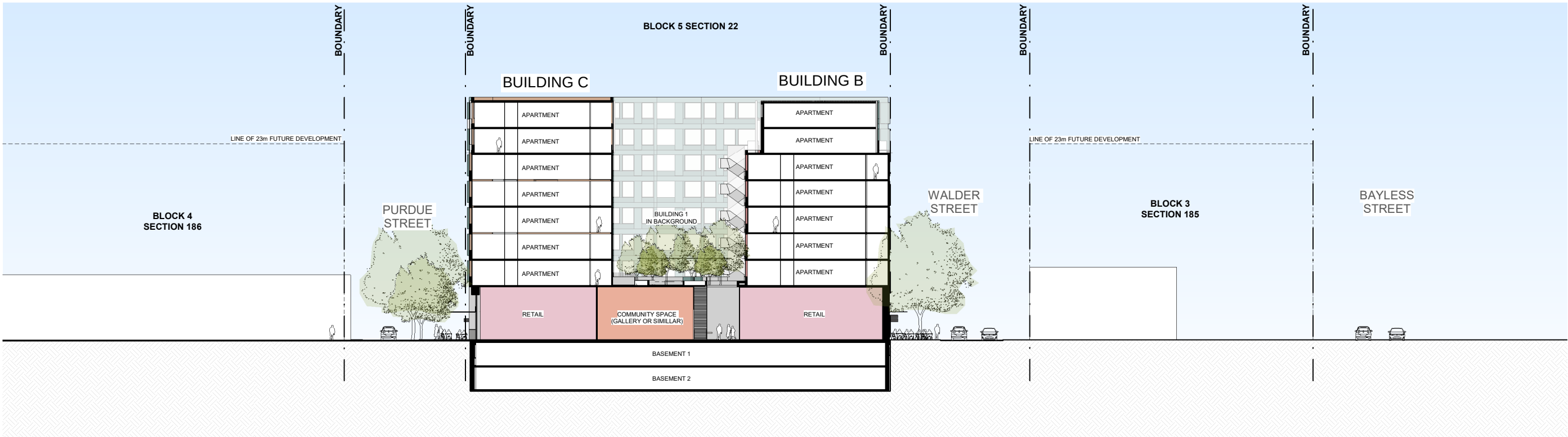
SECTION AA
