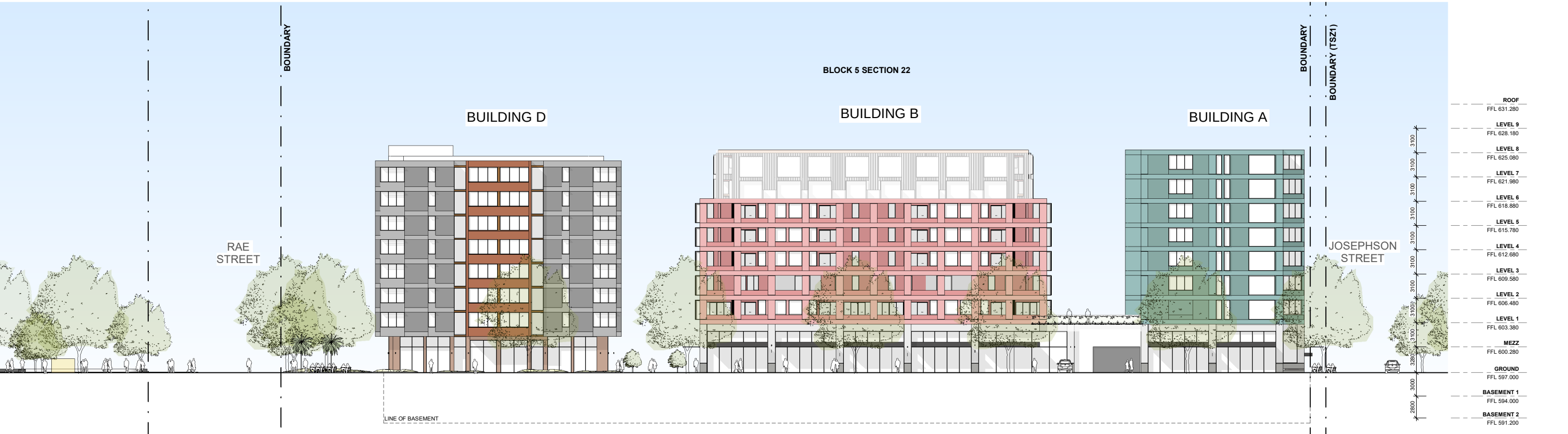
NORTH ELEVATION - WALDER STREET
