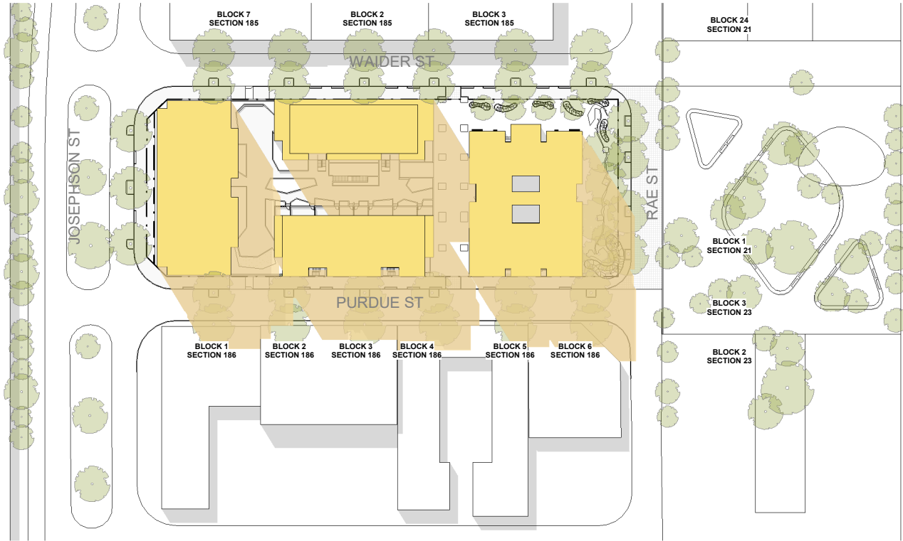
SHADOW DIAGRAM - EQUINOX - 3PM
