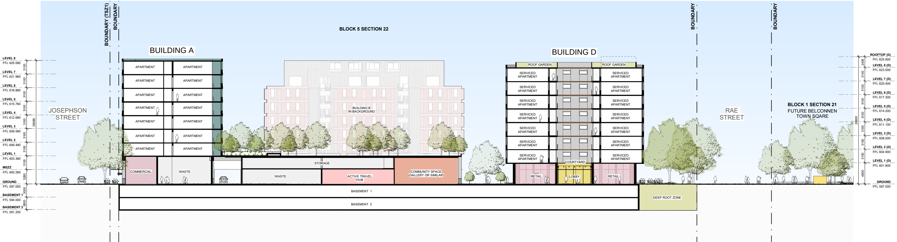
SECTION BB
